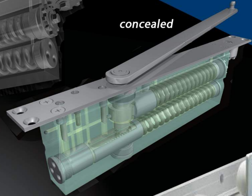
dual cylinder mechanism
